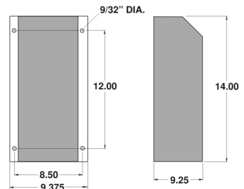
091-143-12 Outline Drawing
